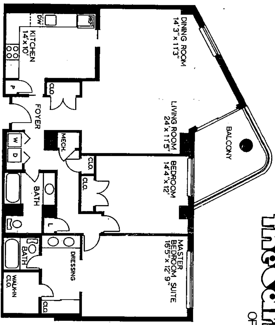
TYPE 2G (Tier 1) 2 Bedrooms, 2 Baths
